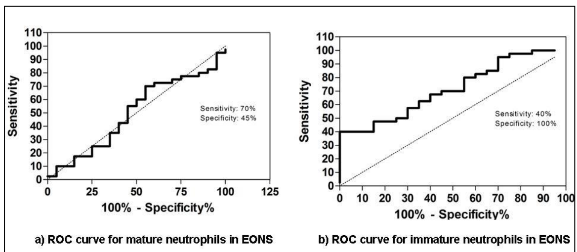
Figure 5: ROC curve for mature and immature neutrophils in EONS
