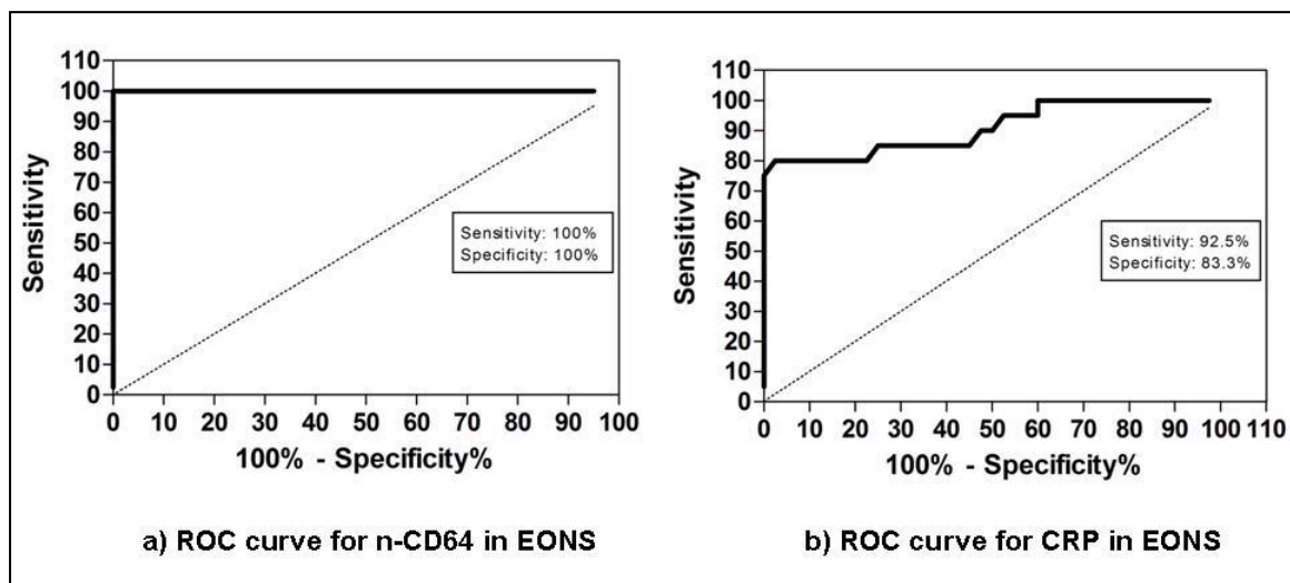
Figure 3: ROC curve for n-CD64 and CRP in EONS
