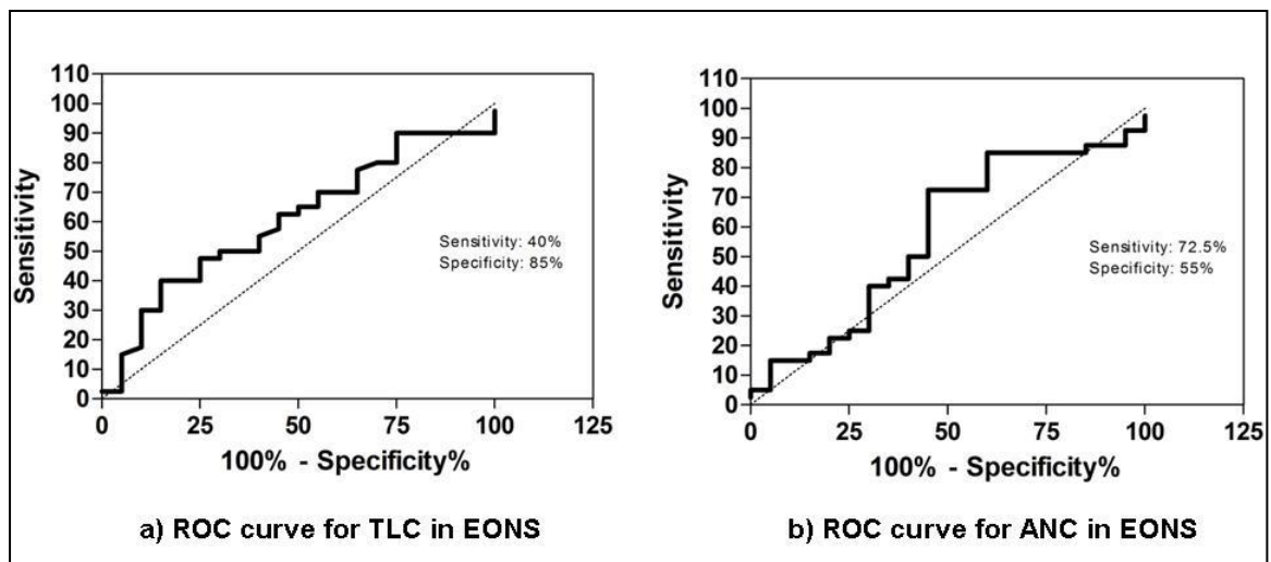
Figure 4: ROC curve for TLC and ANC in EONS
