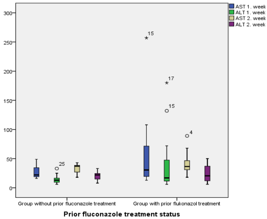
Figure 2. Changes in the serum AST and ALT in the first and second weeks in groups with and without fluconazole treatment.
